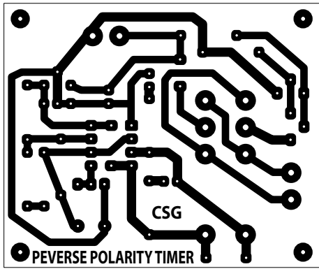
COPPER SIDE 50X60mm
